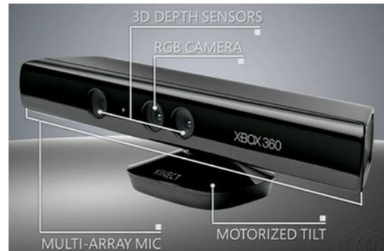
Figure 3. Locations of the various components. Depicted are the locations of the components that make up the Kinect game sensor.
